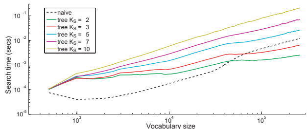
Fig. 7. Performance of the visual vocabulary for the naive method (dashed line) and the tree-based method (solid lines). The parameter K_S refers to the maximum number of children explored at every tree node (maximum is 10).
