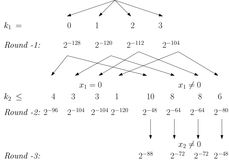
Figure 5: Case Analysis for wF-256
