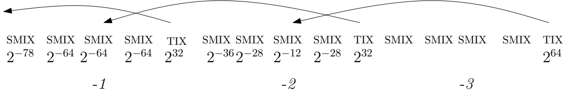
Figure 8: Internal Collisions in F-512 with Free Message Modification upto 6 SMIXes
