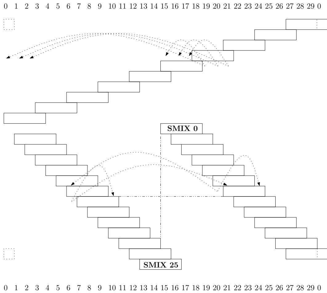
Figure 3: The Final Round \mathbf{G} (in sliding window format)
