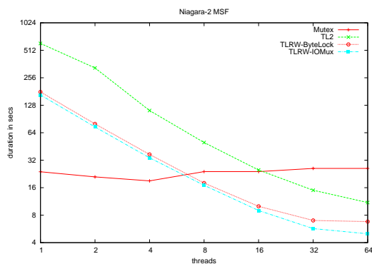
Figure 6: Latency (lower is better) of the transacted MSF application of Kang and Bader.
