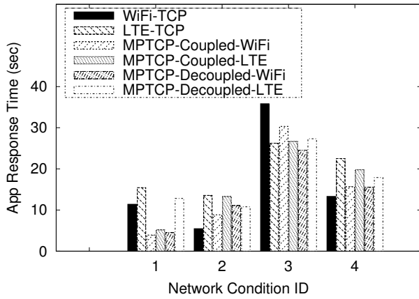
Figure 20: Dropbox app-response time under different network conditions.
