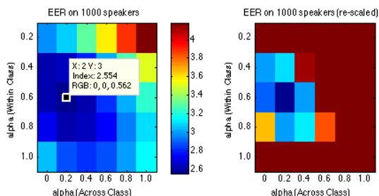
Figure 5: Heatmaps showing the result of independently optimizing the adaptation parameters, \alpha . Both plots involve the same raw data but different color scalings to illustrate the range of \alpha that is appropriate for domain adaptation.
