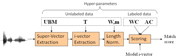
Figure 1: High-level diagram of i-vector system showing all hyper-parameters and which, respectively, require labeled and unlabeled data to train.
