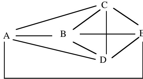
Complete Undirected Graph
