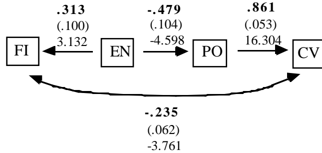
Figure 26. Estimated Alternative Model
