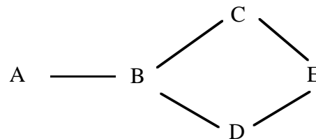
Figure 32: A trace of the adjacency stage of the PC algorithm
