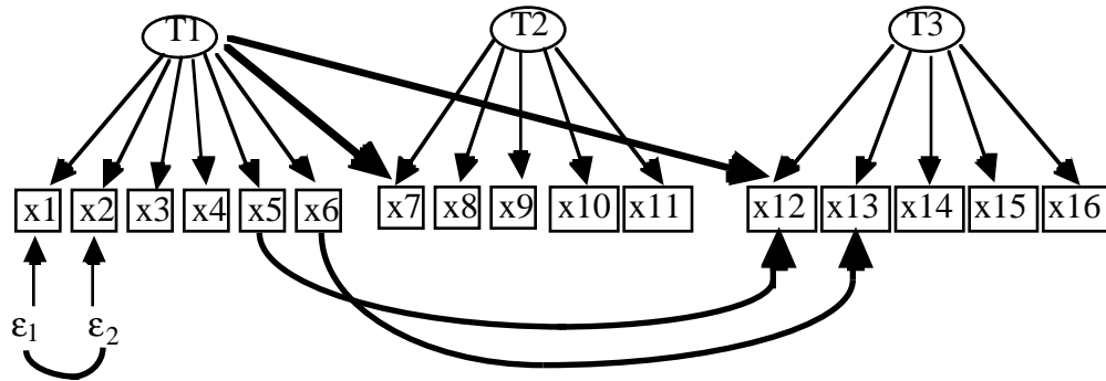
Figure 20: Population Measurement Model
