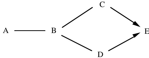
Figure 33. Final Pattern Output by PC.
