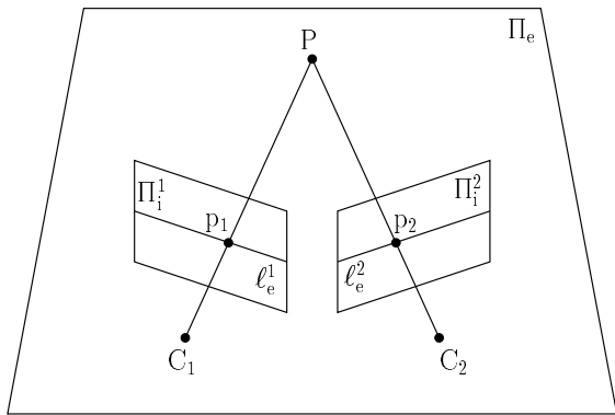
Figure 2: Epipolar geometry.
