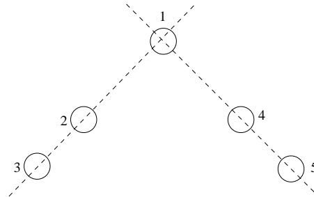
Figure 8: Five receivers on a compass forming two perpendicular receiver-triplets, which are used to unambiguously infer the heading with respect to a beacon.
