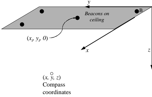
Figure 9: The coordinate system used in Cricket; the beacons are configured with their coordinates and disseminate this information on the RF channel.
