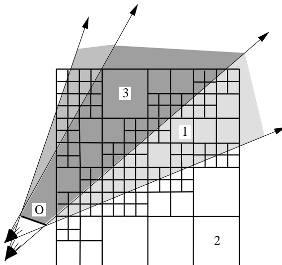
Figure 10: kD-tree nodes classified with respect to a single occluder (O) and two consecutive viewpoints. For clarity, subdivision in the kD-tree is assumed to occur at the center of each kD-tree node.
