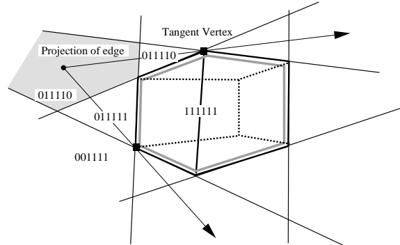
Figure 8: The projection of a box with respect to the origin (shown in 2D). Regions induced by extended silhouette edges are numbered using 6-bit codes consisting of the signs of dot products with (directed) silhouette lines. Tangent vertices are determined by the location of the occluder edge’s projection.
