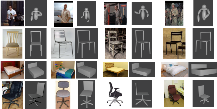
Fig. 10. Visualization of 3D reconstruction results. We render objects using Blender .
