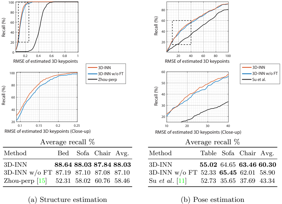
Fig. 7. Evaluation on the IKEA dataset [14]. (a) The accuracy of structure estimation. RMSE-Recall curved is shown in the first row, and zoomed-views of the dashed rectangular regions are shown in the second row. The third row shows the average recall on all thresholds. (b) The accuracy of pose estimation.
