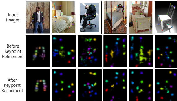
Fig. 5. 2D keypoint predictions from a single image, where each color corresponds to a keypoint. The keypoint refinement step cleans up false positives and produces more regulated predictions.
