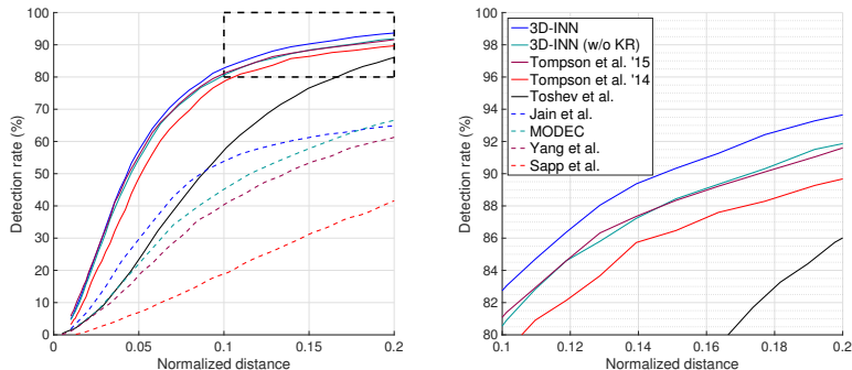
Fig. 4. PCK curves on the FLIC dataset. 3D-INN performs consistently better than other methods. Without keypoint refinement, it is comparable to Tompson et al. [32]. A zoomed view of the dashed rectangle is shown on the right.
