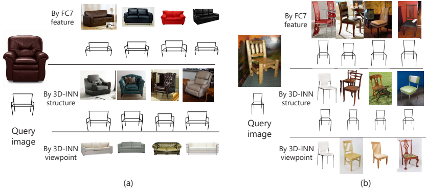
Fig. 11. Retrieval results in different feature spaces. 3D-INN helps to retrieve objects with similar 3D structures or similar viewpoints.
