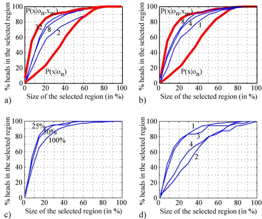
Figure 17. Quantifying the ability of contextual features to reduce the size of the search region as a function of (a) number of contextual features ( D = 2, 8, 32 ). The thick lines show the lower and upper bounds in location priming (lower = p(x|o) , upper = p(x|o, x_m) ). (b) Performance as a function of the number of clusters. Graph (c) shows performances for the top 25% and 50% of images with the lowest \sigma_r^2 . Graph (d) compares performances across the four object classes (1-people, 2-furniture, 3-vehicles and 4-vegetation).
