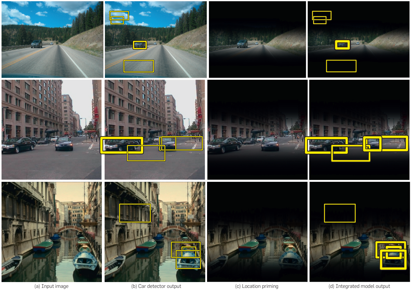
Figure 6. (a) Three input images. (b) Top four detections from an object detector based on local features. The thickness of the boxes is related to the confidence of the detection. (c) Predicted location of the car based on global features. (d) Combining local and global features.
