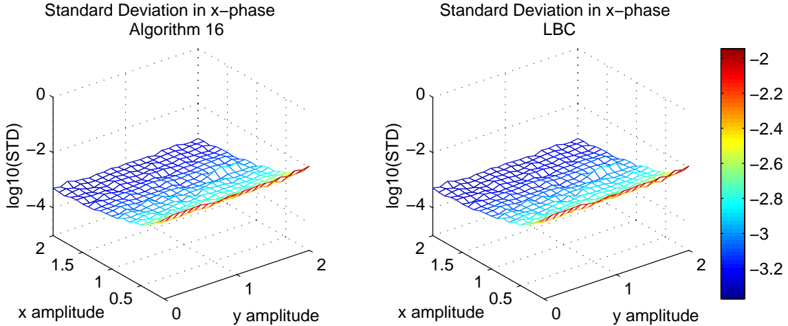
Figure 5-14: The standard deviation of phase errors for algorithm 16 for simulations of the fatigue test structure image. The simulations are described in Section 5.5.1 and Section 5.5.1
