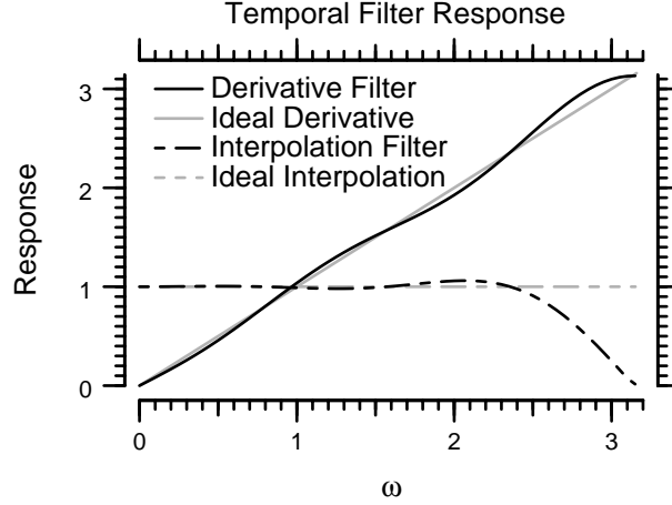
Figure 5-5: Frequency response of the 8-point temporal derivative and temporal interpolation filters.
