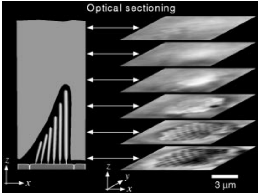
Figure 2-1: Illustration of optical sectioning. A three-dimensional volume image is generated by capturing a sequence of two-dimensional images at different focal planes. The focal plane is adjusted by application of a voltage to a piezo that translate the lens along the optical axis.
