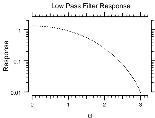
Figure 5-9: Frequency Response of the four point low-pass filter.
