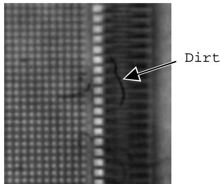
Figure 2-2: A example of fixed-pattern noise due to dirt on a lens. The image is one in a sequence of images of part of a moving gyroscope (Draper Labs, Cambridge MA). The dirt, indicated by the arrow, was observed to remain stationary while the gyroscope moved underneath it.
