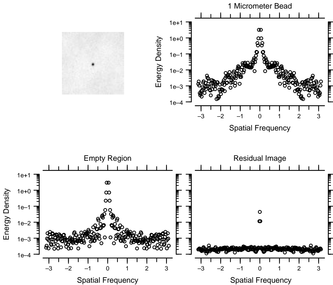
Figure 2-3: Top left: two-point corrected, 256x256 pixel image of a 1\ \mu\text{m} diameter bead. Top right: average power spectrum of the bead image after two-point correction. Bottom left: average power spectrum of 256x256 region containing little visible structure after two-point correction. The region was located several hundred pixels away from the bead. Bottom right: average power spectrum of residual images. These images are the results of subtracting the average image of the bead from each image of the bead as described in Section 2.3.1.
