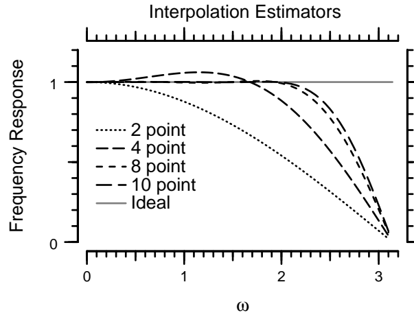
Figure 5-2: Frequency response of interpolation filters created using the Parks McClellan algorithm with weighting function as described in Figure 5-1. The filter with support 2 is used in the first difference algorithm.
