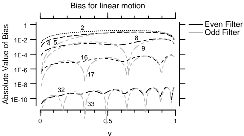
Figure 5-4: Error in the estimate of motion between two images using the data in many images. The sequence of images consists of \sin 2(i - vt) . The bottom two traces use 32 images and 32 points in space and 33 images and 33 points in space to calculate each derivative. The next highest traces use 16x16 and 17x17 regions in space-time. The number of images and pixels used to calculate each derivative in an estimator is shown next to its trace. The highest trace is the first difference algorithm with a support of 2x2.
