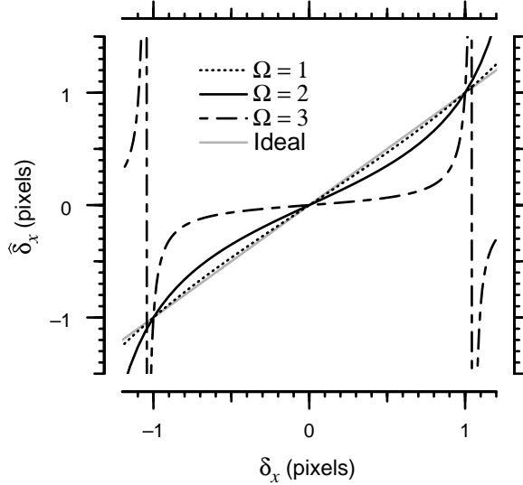
Figure 4-3: Estimates \hat{\delta}_x of the displacement \delta_x between two sinusoidal images using the first difference estimator. The curves illustrate gradient-based estimates of displacement (4.11) for sinusoidal images with frequencies \Omega , where \Omega = \pi is the Nyquist frequency.
