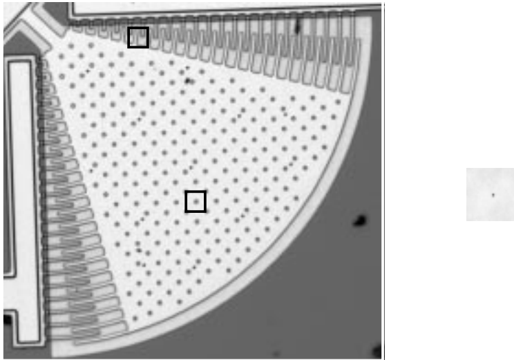
Figure 7-1: Image of the fatigue test device on the left and the bead on the right. For both images, motion was parallel to the bottom of the image. The two boxes on the fatigue test device indicate analysis regions. The analysis region on the combs of the fatigue test device was examined only in Section 7.4.2 for a consistency check.
