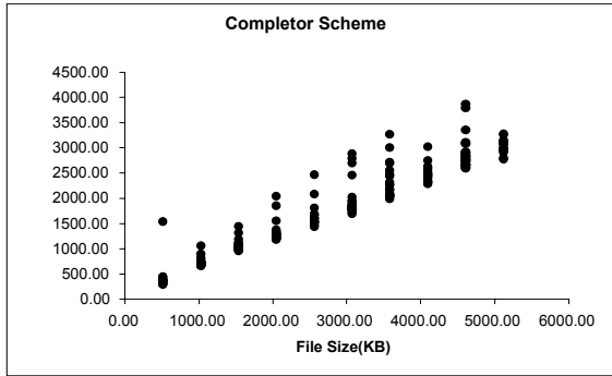
Figure 7: Variability in the file download times due to the last block problem in the greedy-completor strategy
