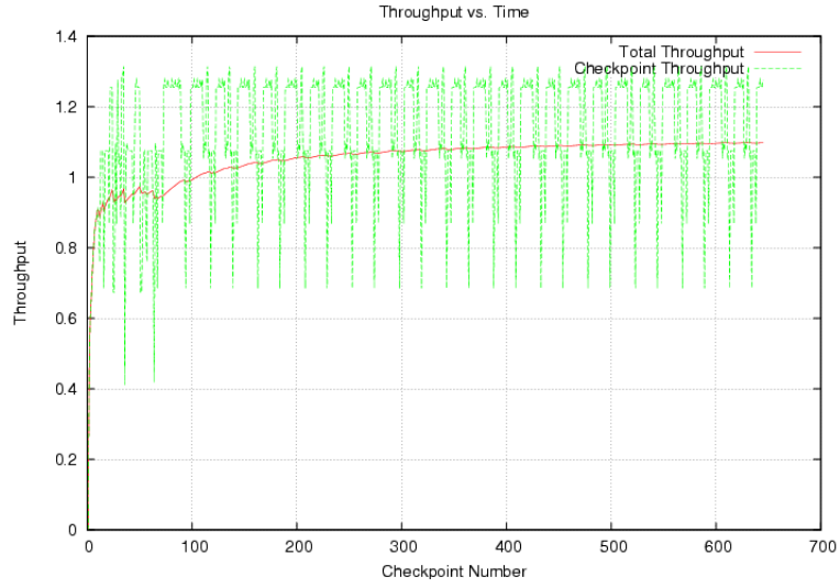
(a) \text{OFFSET}=.2 , \text{OFFSET\_SCALE}=.25
