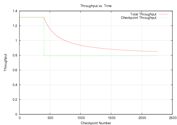
(c) dynamic (brute force)
