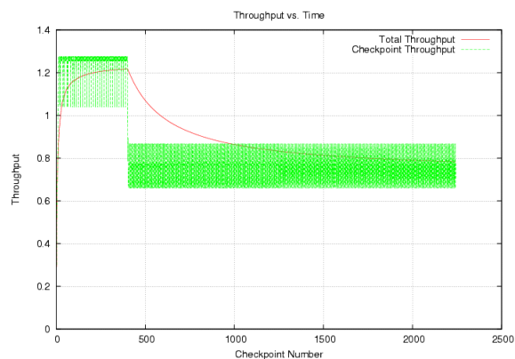
(a) market (brute force)
