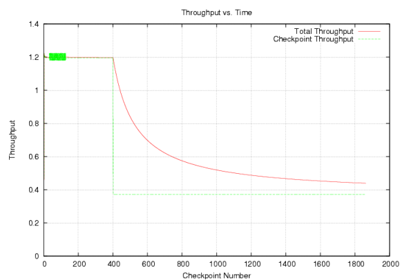
(b) static (brute force)
