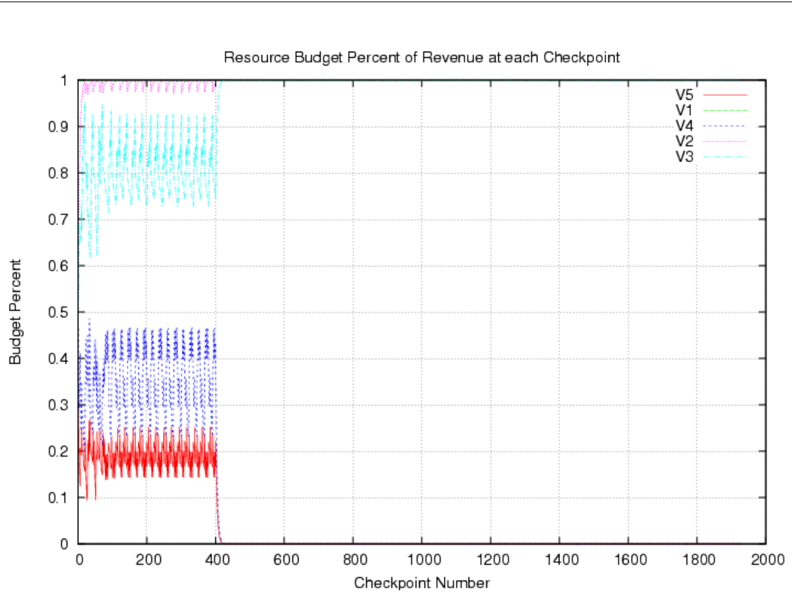
Figure 5-10: Resource budget percentage of revenue for market runtime handler with singular load change
