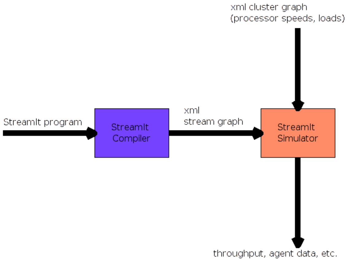
Figure 4-1: High-level functionality of the StreamIt simulator. A modified version of the compiler generates the stream graph xml file. That, along with the cluster graph xml file, are input to the simulator.
