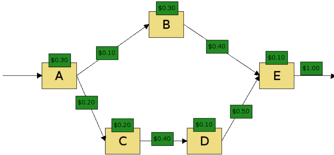
Figure 4-4: Monetary distributions. Lettered boxes are filters. Green boxes represent revenue distributions. Green boxes just above the filters are the associated resource budget. The total sum of all the resource budgets will always add to the revenue of the final vertex, which is arbitrarily set to 1 monetary unit. Revenue allocation occurs in sequence from the final vertex upstream to the start vertex.
