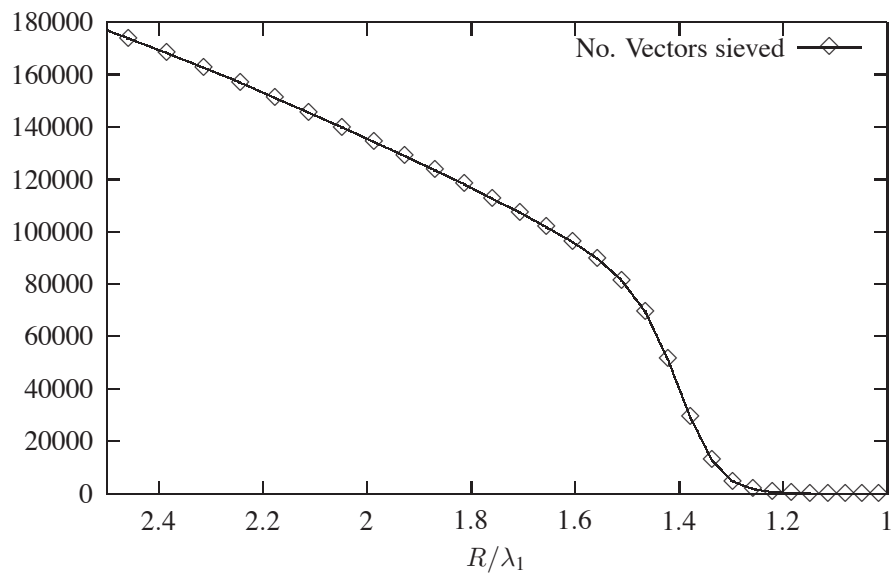
Figure 2. Number of collisions observed.
