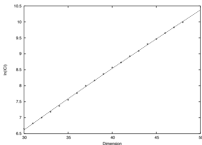
Figure 3: Logarithm of the maximal number of centers used in any iteration of the sieve algorithm, experimentally.
