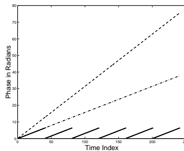
Figure 2: Schematic of phase (in radians), unwrapped phase and doubled unwrapped phase, for a single channel [4].
