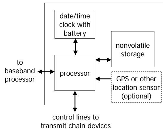
Figure 3. Components of the lease subsystem for an integrated mobile device. Local nonvolatile storage holds the current leases and crypto keys. An optional location sensor can support location-limited leases.
