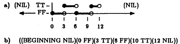
Figure 1. a) Piecewise-constant partial function mapping time into boolean values; b) corresponding LISP representation (GRAPH).
