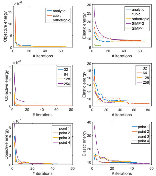
Fig. 9. Convergence tests. Variation of the objective energy ( left ) and the elastic energy right of a beam being optimized for minimum compliance as the optimization progresses. The convergence plots correspond to the beam of Figure 8 when optimized using different material spaces ( top ), different resolutions for the beam lattice ( middle ) when using cubic microstructures, and different initial material properties for the cubic microstructures ( bottom ).
