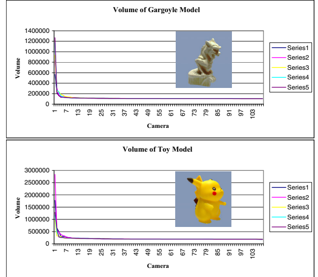
Figure 12: The volume of the visual hull as a function of the number of images used to construct the visual hull.
