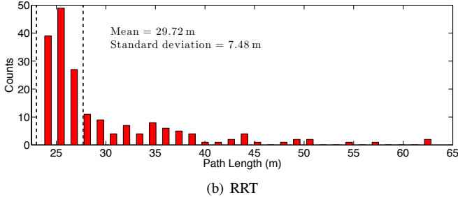
Fig. 4. Histogram plots of the executed path length for simulations of (a) the RRT* and (b) the RRT. The vertical dashed lines in (b) depict the range of path lengths that result from the RRT* planner.
