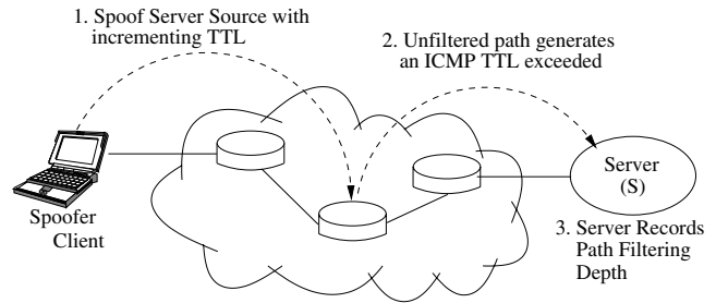
Figure 5: Example of tracefilter second iteration: 1) Client sends packet with TTL=2, src= S , dst= S + 1 , payload length=2. 2) With no filters along first two hops, the packet expires, generating an ICMP TTL exceeded message to our server S . 3) The server records the originating TTL of 2 by decoding the ICMP message body’s UDP length. Client tests entire path; the largest originating TTL is one less filtering point.
