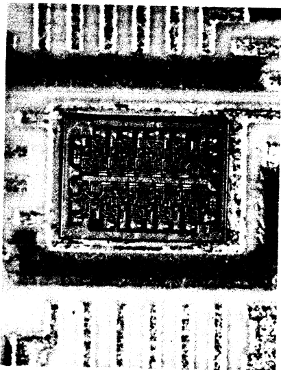
Figure 10: Micrograph and photo of TV monitor image of integrated circuit chip with bright aluminium border. Note high-lights on pads caused by probing electrodes.
