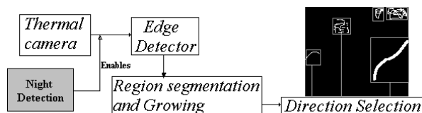
Figure 9: Night navigation algorithm
