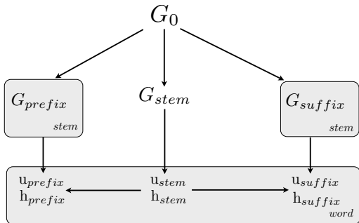
Figure 7. Plate diagram of the decipherment model. The base distribution G_0 defines character probabilities over string-pairs based solely on character-level correspondences. The morpheme-pair distributions G_{stem} , G_{prefix} , G_{suffix} directly assign probabilities to highly frequent morpheme pairs. Each stem pair provides a separate distribution over prefix and suffix pairs.
