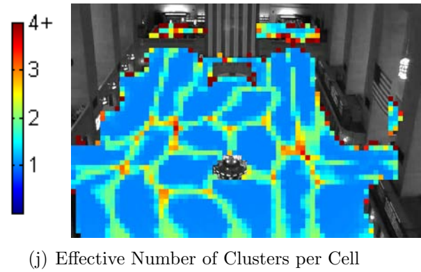
Figure 4-2: Activity Modeling with Feature Points : In Fig. 4-2(a), we show the learned activity cluster mixing weights, after sorting them. In Fig. 4-2(b), we show the marginal distribution of all observations (quantized location and moving direction of a tracked feature point) in the dataset. The hue mask in Fig. 4-2(c) encodes direction, and its alpha matting with respect to the background image encodes the observation frequency. Fig. 4-2(d)–4-2(i) show the six most highly weighted clusters. Note that although each cluster does have good spatial compactness, it captures motion in all directions. The model is unable to learn overlapping clusters where people are traveling on different paths. Except for a few of the low-weighted ones (which are not shown here), the remaining 17 clusters are qualitatively similar. In Fig. 4-2(j), we see that there is only a single cluster representing motion at most locations on the concourse floor.
