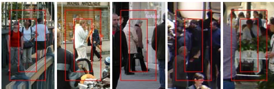
Figure 3-17: Positive Training Images from the INRIA-new Dataset : These images are people that were excluded from the INRIA-orig dataset. The outer red box shows the detector window boundary. The inner red box shows the canonical pedestrian size within a window.
