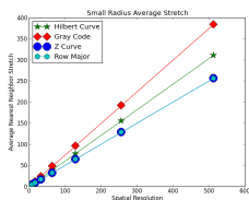
(a) Standard ANNS
