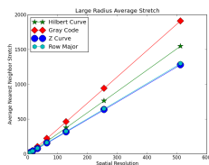
(b) Large Radius ANNS
