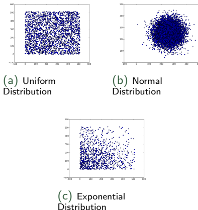
Figure : This figure shows examples of the two dimensional probability distributions considered in this paper.
