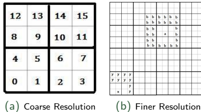
Figure : Interaction Lists: Figure showing two partitioned spatial resolutions. In the coarse resolution image (a), the interaction list of node 0 is \{2, 3, 6, 7, 8 - 16\} , or every node that it not in its quadrant. However, the interaction list of node 6 is \{0, 4, 8, 12, 13, 14, 15\} . At the finer resolution, nodes in the interaction list of x are marked with y and nodes in the interaction list of a are marked with b .
