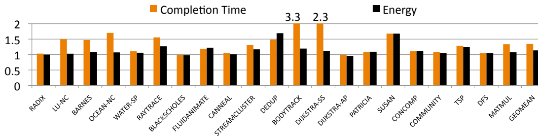
Figure 14: Ratio of Completion Time and Energy of Adapt_{1-way} over Adapt_{2-way}
