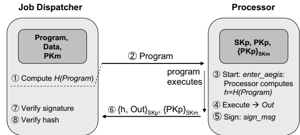
Figure 4: Certified execution for distributed computation.
