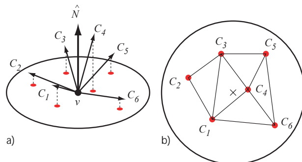
Figure 1: Delaunay triangulation of visible views. (a) Viewing directions of visible camera views ( C_1 - C_6 ) at vertex v are first projected onto the tangential plane of v . (b) Then a 2D Delaunay triangulation of the projected views is constructed.
