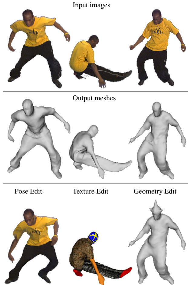
Figure 1: Our methods for pose tracking and non-rigid shape matching make it possible to extract a mesh animation with full correspondence (middle row) from multi-view video data (top row), allowing easy editing of pose, appearance, and character geometry (bottom row).
