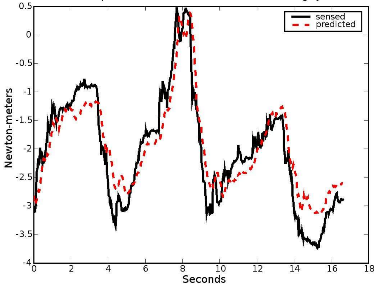
Torque Prediction for Ballistic Reaching [Joint0]
