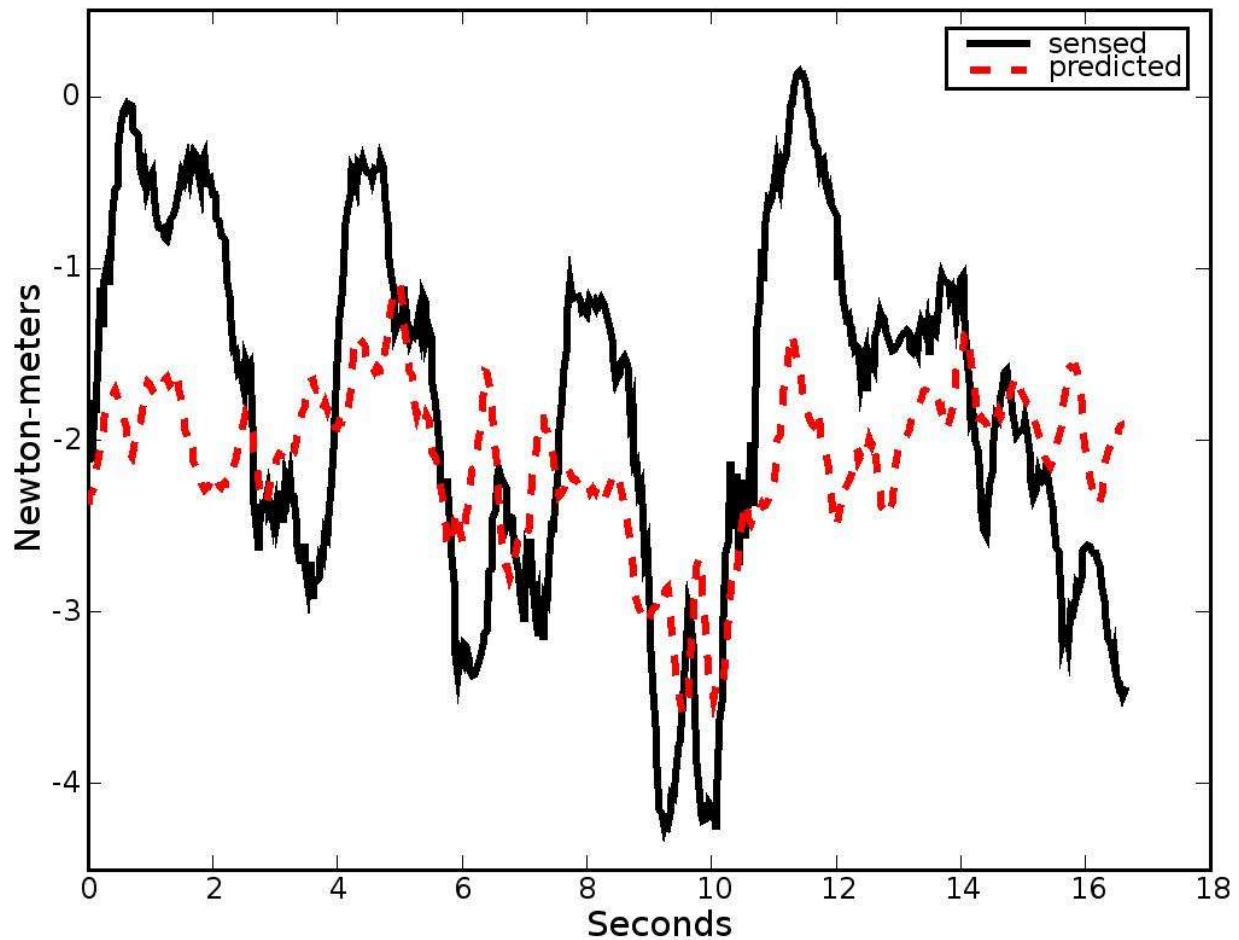
Torque Prediction for Exo Reaching [Joint0]
