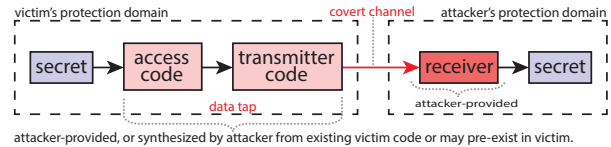
Fig. 1. Attack Schema: an adversary 1) accesses a victim’s secret, 2) transmits it via a covert channel, and 3) receives it in their own protection domain.
