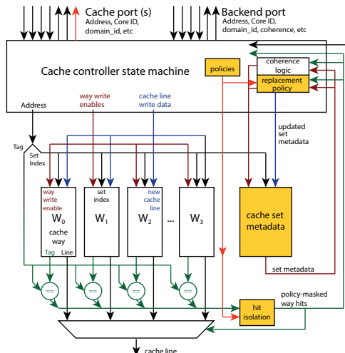
Fig. 4. A Set-Associative Cache structure with DAWG.
