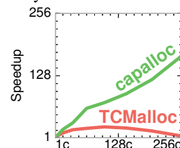
Fig. 4. des speedup on 1–256 cores, with different allocators.
