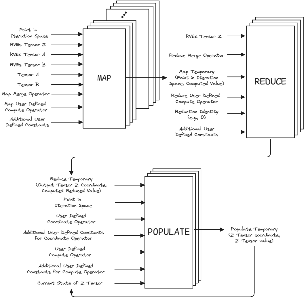
Fig. 16. Execution flow of an EDGE Einsum evaluated over the entire iteration space. The diagram illustrates how points in the iteration space are projected through rank variable expressions into tensor coordinate spaces, and how values are produced and propagated across all points.
