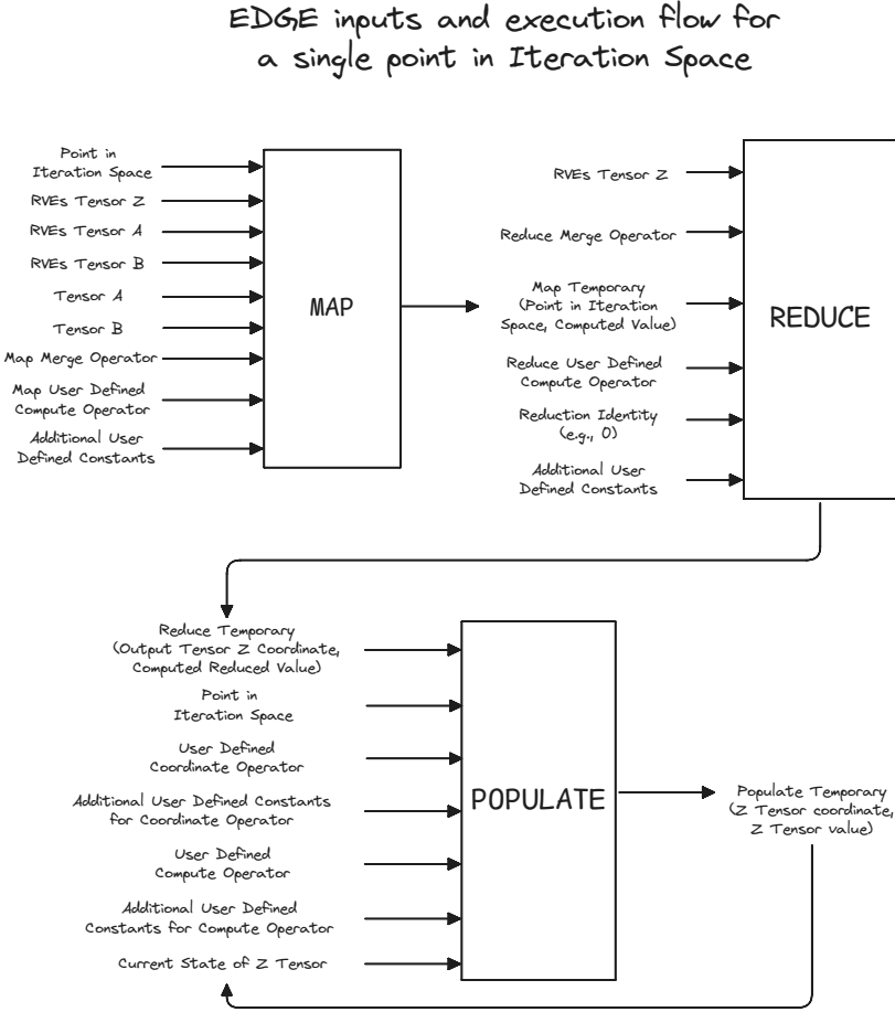
Fig. 15. Execution flow of an EDGE Einsum with input tensors A , B and output tensor Z , evaluated at a single point in the iteration space. The figure highlights how a single point in the iteration space passes through rank variable expressions to produce coordinates in the tensor coordinate space, and how those coordinates produce a value in the data space.
