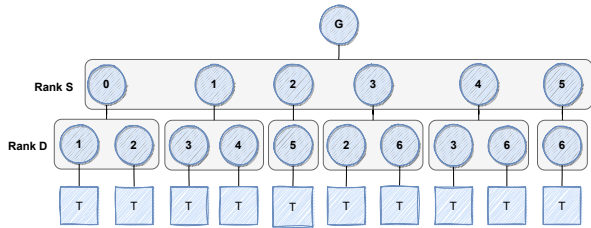
(b) Here, we express G as a tensor where vertex IDs are now numerical and the leaf values indicate whether there is an edge connecting vertex s to vertex d , where T is True and F (the empty value) is False.
