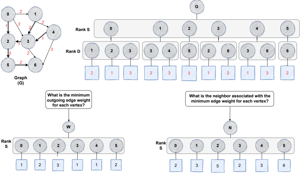
Fig. 10. (Top Left) A directed graph, G , with edge weights in red. (Top Right) A fibertree representation of the graph, G_{s,d} . The leaf values contain the edge weight. (Bottom Left) Resulting tensor, W , that records the minimum outgoing edge weight for each vertex in the graph (see Equation (42)). (Bottom Right) Resulting tensor, N , that records the destination vertex ID of the outgoing edge with the minimum edge weight.
