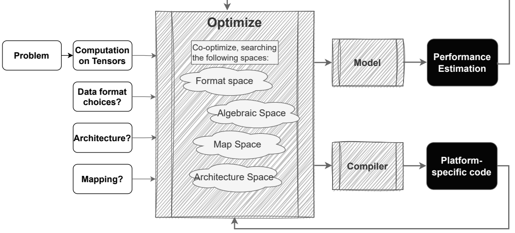
Fig. 5. Our view of the complex design space in tensor algebra. Shaded boxes indicate processes (searching the space), white/black boxes indicate inputs/outputs to the system. Given a problem, a tensor algebra implementation must try to optimize across the possible data formats, possible algebraic variants of the computation, and the mapping space, as well as selecting the best architecture. Tools tend to either model performance (for domain-specific accelerators), or generate platform-specific code. The results may be used to search for better points in the implementation space.
