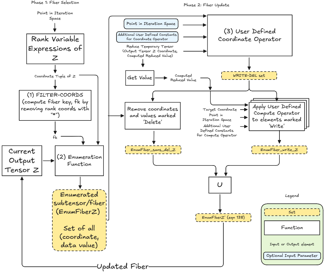
Fig. 19. POPULATE: given the current state of the output tensor Z and an incoming REDUCE TEMPORARY element, POPULATE selects the corresponding fiber (using the fiber key derived from “*”-marked ranks), applies a user-defined Coordinate operator to produce a WRITE/DELETE/NONE action label for each coordinate in the fiber, and then applies the Compute operator to produce the new values at WRITE locations. The updated fiber replaces the original in Z .
