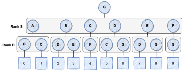
(a) Here, we express G as a tensor where the leaf values contain edge IDs.
