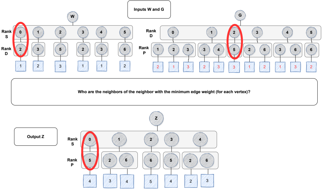
Fig. 11. The two input graphs, W and G , involved in the Einsum expression that finds the neighbors of the minimum-weighted vertex (see Equation (44)). Red circles indicate the intersection of the d rank, when s = 0 , between W and G . The result is in output tensor Z . Z does not contain vertex s = 5 as its minimum-weighted neighbor, vertex 6, has no neighbors. The values in Z indicate the cost of going from vertex s to vertex p through the minimum-weighted neighbor of s .
