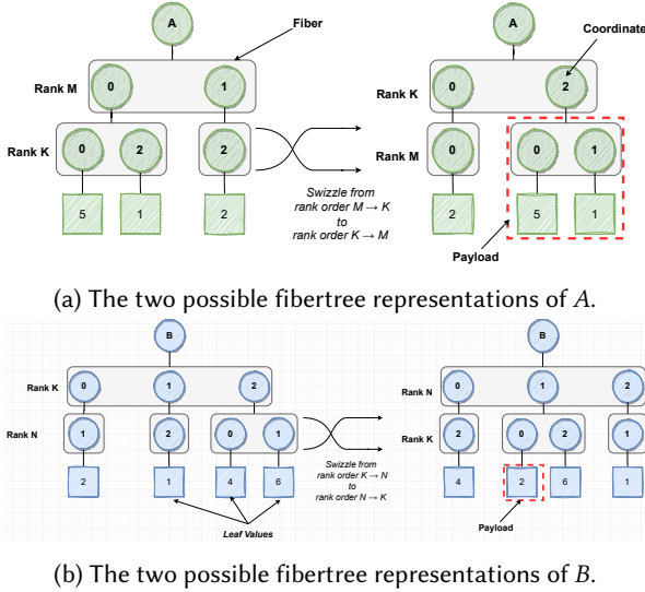
Fig. 2. Fibertree representations of the uncompressed tensors in Figure 1.
