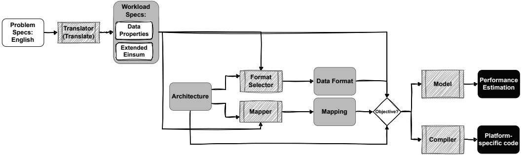
Fig. 6. One common approach to factoring the design space in tensor algebra. Shaded boxes with side borders indicate processes , plain shaded boxes indicate specifications for a concern, while white/black boxes indicate inputs/outputs. Tools search subspaces to select a point within that space (e.g., a mapper selecting a mapping), then pass the selected point to the next subspace to inform its search (e.g., given a mapping, select the best data format).
