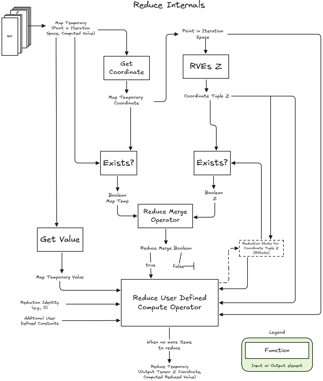
Fig. 18. REDUCE: for each output tensor coordinate cs^Z , REDUCE combines the current reduction state RState(cs^Z) with the incoming MAP TEMPORARY value using the user-specified Merge and Compute operators. The result updates RState(cs^Z) . When no further MAP TEMPORARY elements remain for that coordinate, RState(cs^Z) contributes a final reduced value to REDUCE TEMPORARY.
