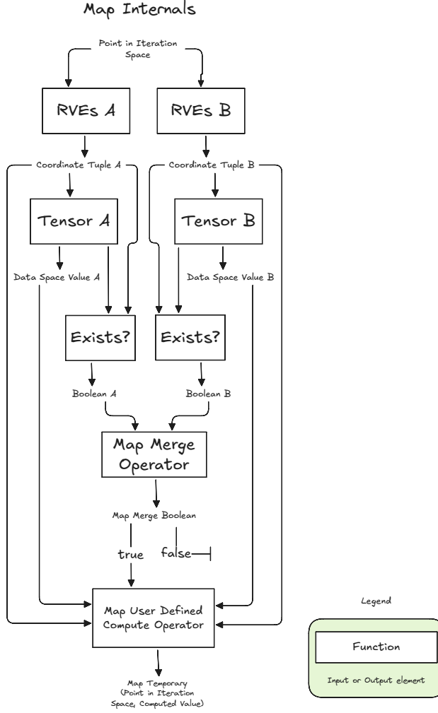
Fig. 17. MAP: Operand values accessed at a point in the iteration space are combined to produce a MAP TEMPORARY, which is then forwarded to the subsequent REDUCE action.
