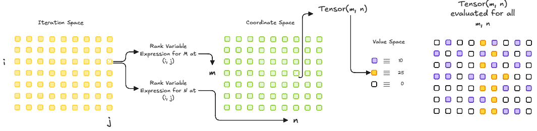
Fig. 14. Two rank variable expressions transform points in the I \times J iteration space to points in the M \times N coordinate space of tensor Tensor . The tensor itself takes a point in the coordinate space to a value in the data space.
