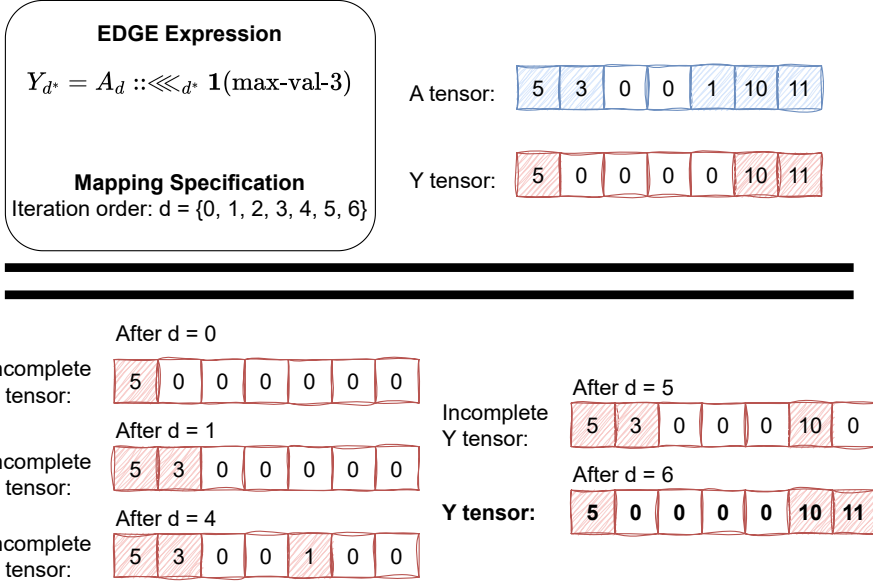
Fig. 12. Top half: An EDGE expression using populate, where Y is a filtered version of A that contains only A 's maximum three values (Equation (46)). We show example input tensors A and Y , and a specific mapping specification on how execution should walk the D iteration space. Bottom half: The state of Y and its mutable d rank after execution has processed certain points in the iteration space.
