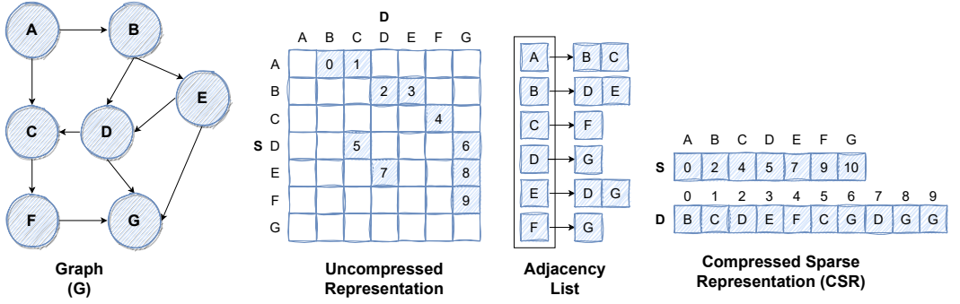
Fig. 3. A directed graph, G , and some representations. The matrix values contain the edge ID, while the vertices are labeled alphabetically.
