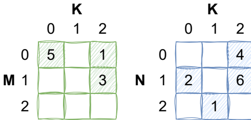
Fig. 1. Uncompressed 2D tensors, A and B , where locations containing zero are treated as empty in this example. This also shows the coordinate spaces of A and B , whose points map to values in each tensor’s data space.
