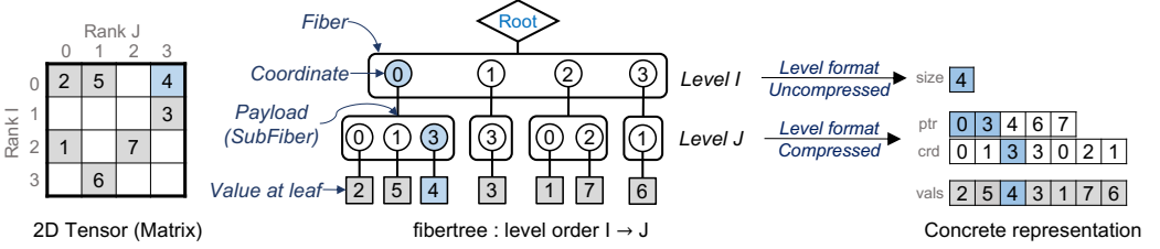
Fig. 10. A traditional sparse matrix, its fibertree abstraction and concrete representation stored in memory.
