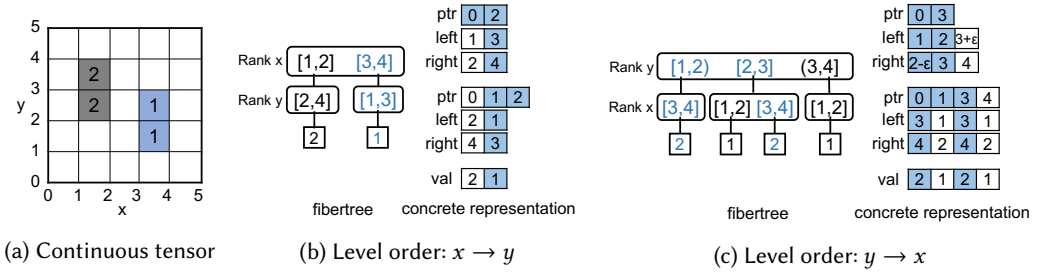
Fig. 13. Two concrete representations based on different level orders. With the level order x \rightarrow y and y \rightarrow x , the alternative representation illustrates how memory usage can be reduced depending on the chosen order.
