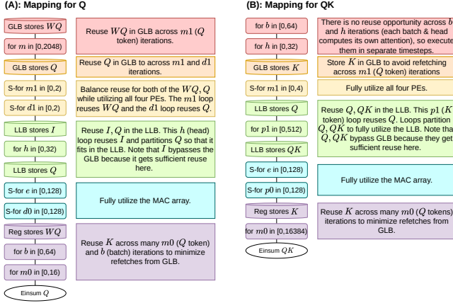
Figure 9: (Left) Mapping for Einsum Q , and (Right) Mapping for Einsum QK , annotated with the goals the mapper is attempting to accomplish at each level. Memory levels are DRAM (omitted), global buffer (GLB), local buffer (LLB), and reg. S-for denotes spatial loops. Notice that there are many tradeoffs to consider, including capturing reuse to minimize refetches, fully utilizing spatial units, and ensuring that no memories are overprovisioned.
