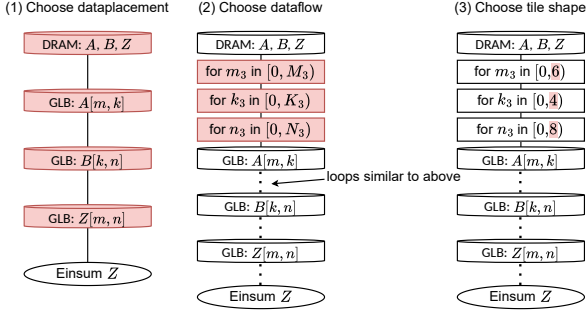
Figure 2: Constructing a mapspace for the Einsum in Eq. 1 by choosing dataplacement, dataflow, then tile shape. The part of the mapping chosen in each step is highlighted in red. In (2) and (3), only some choices are shown; similar choices must be made for parts in ellipses.
