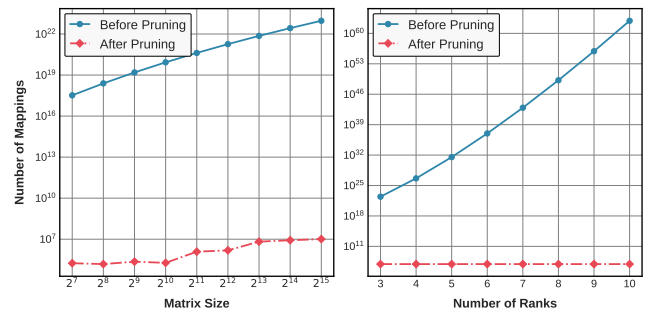
Figure 7: Mapspace size scaling, with and without pruning, for matrix multiplies on a TPU-v4i-like accelerator. (Left) Mapspace size scaling with matrix size, with three total ranks ( M , N , and K ). (Right) Mapspace size scaling with the number of ranks, with matrix dimensions M = N = K = 16384 and additional size-1 ranks added to the weight tensor. As mapspace expands, pruning becomes more effective, keeping search size tractable even for very large mapspaces.
