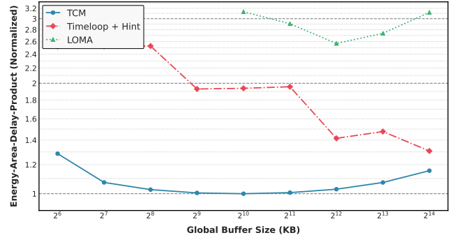
Figure 10: TCM accurately informs design space explorations, while prior works do not because mapper limitations hide the effect of architecture changes.
