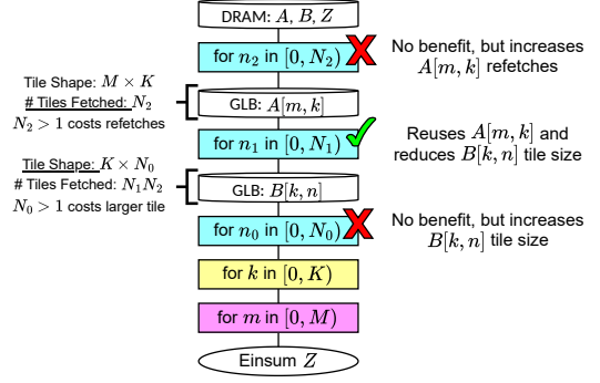
Figure 4: A mapping with non-helpful loops. Notice that the n_2 and n_0 loops both have costs (more fetches, more tile size) but no benefits (lower fetches, lower tile size). The n_1 loop is strictly better than either. Loop pruning will eliminate the n_2 and n_0 loops while keeping the n_1 loop.
