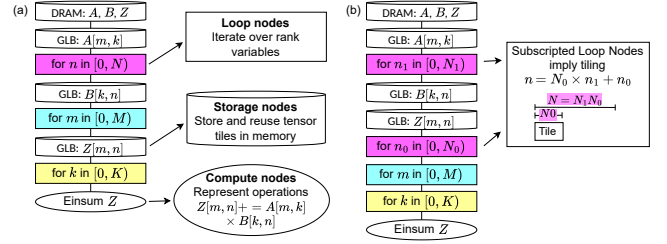
Figure 1: (a) An example LoopTree, the different types of nodes, and their meaning. (b) An example LoopTree with tiling.
