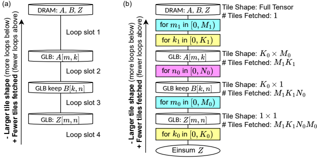
Figure 3: (a) An example dataplacement and slots where loops may be inserted. (b) An example mapping using the dataplacement, including tile shapes and numbers of tiles fetched. Dataplacement shows the trade-off between tile size and number of tiles fetched: Storage nodes higher in the dataplacement reduce fetches, but can increase tile size.
