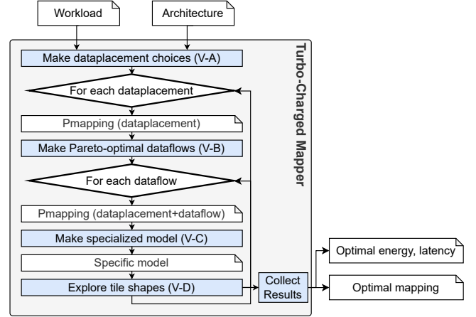
Figure 5: Overview of TCM. Each mapper process (in blue) is explained in detail in the sections in parentheses.
