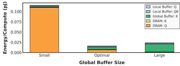
Figure 11: TCM balances the energy of multiple memory levels to yield low-energy accelerators. The optimal design uses a moderately-sized global buffer to reduce DRAM accesses while costing moderate global buffer access energy. To make differences clearer, we omit irreducible costs of MACs and writeback of the output tensor QK to DRAM (which TCM does only once), noting that Fig. 10 includes all components.
