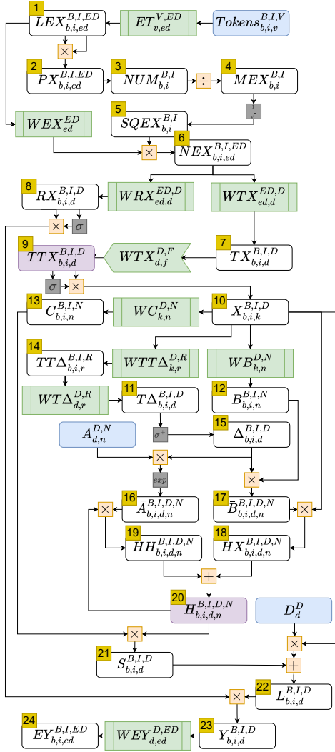
Fig. 1: Overview of the cascade execution flow for Mamba. Rounded, rectangular boxes are tensors, with the rank names (and shapes) in superscripts, and the corresponding rank variables (tensor indices) in the subscripts [30]. Each Einsum is labeled with a number (yellow box) on its output tensor. Colors represent the following: (a) blue: input tensor, (b) green: GEMM with a weight tensor, (c) purple: tensor with recurrent accesses (e.g., H_{i-1} ), (d) light orange: elementwise/broadcast operation, (e) dark grey: unary and nonlinear functions.
