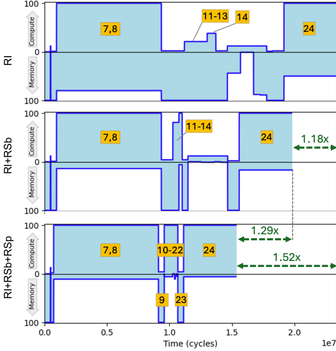
Fig. 10: Roofline utilization over time of single Mamba layer for different fusion strategies. All assume algorithmic minimum accesses on intra-Einsum traffic. Successively applying fusion variants reduces the overall number of fusion groups and improves overall latency.
