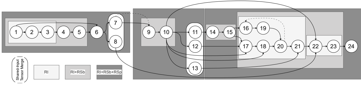
Fig. 9: Fusion opportunities in the Mamba cascade. Each node denotes an Einsum, and directed edges indicate data dependencies between their input and output tensors. Dashed arrows indicate recurrent or correlation Einsums.
