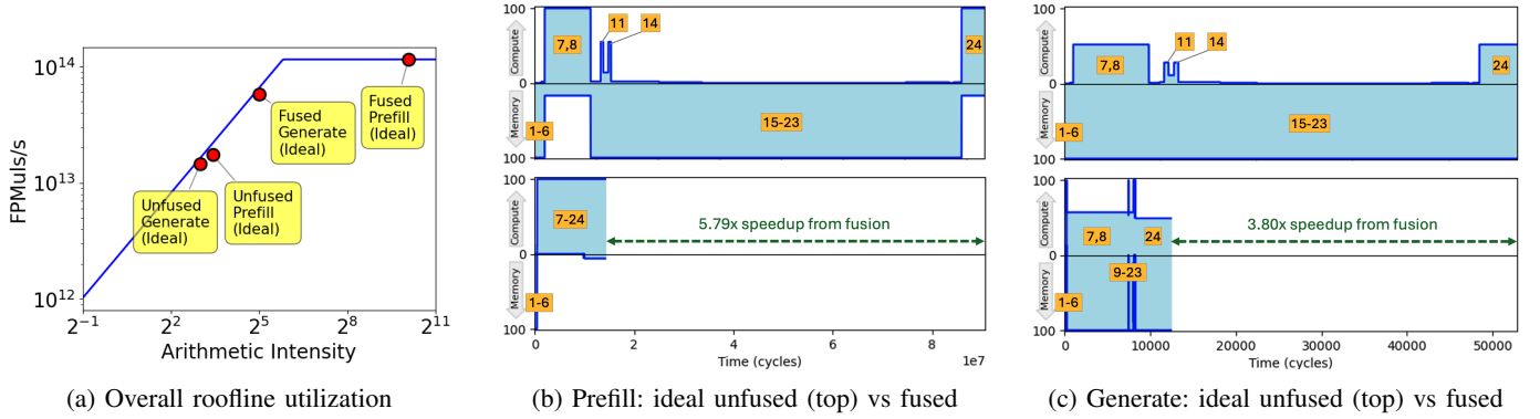
Fig. 2: Overall roofline plot (a) confirms that unfused operations are memory-bound, but does not give insight into Einsums’ relative weighting. Plotting detailed roofline utilization over time for a single layer demonstrates that (b) unfused prefill alternates between compute-bound and memory-bound Einsums, whereas (c) decode does not have enough reuse to reach the compute-bound in any Einsum. Phase labels in yellow correspond to the Einsum numbers in Figure 1. Ideal fusion would eliminate all inter-Einsum traffic, resulting in significant increases to intensity, as shown in the bottom figures.
