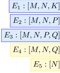
(c) Final mapping into two fusion groups
