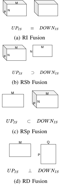
Fig. 3: Examples of how each fusion class transforms an upstream iteration space to a downstream iteration space.
