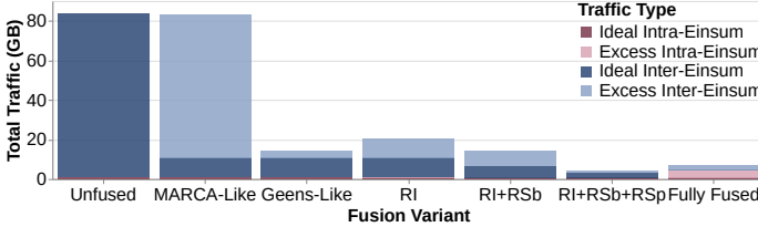
(b) Decode / Token generation (B=64, I=1).
