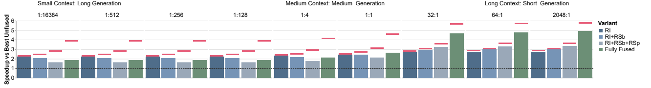
Fig. 12: End-to-end performance across the different variants for the mamba-370m model [59]. In red is the ideal performance (best-case scenarios with algorithmic minimum accesses). Bars indicate the achieved performance.
