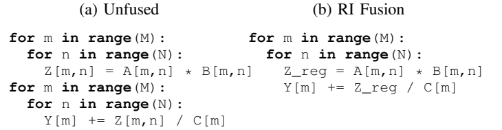
Fig. 4: Unfused to RI fusion. Both Einsums share the same iteration space.
