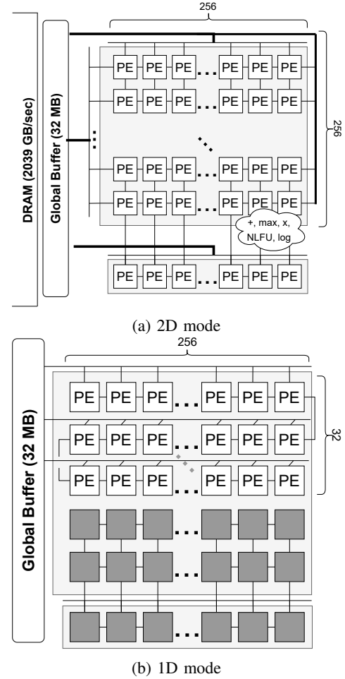
Fig. 11: Mambalaya’s reconfigurable architecture, with the (a) 2D array in 2D mode and (b) the 2D array in 1D mode. The 1D 256-PE array also connects to the first row of the 2D array.
