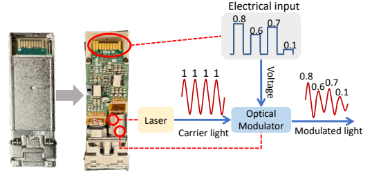
Figure 1: Amplitude modulation in a commodity transceiver.
