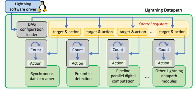
Figure 11: LIGHTNING's count-action abstraction enables implementing runtime reconfigurable modules on its datapath.
