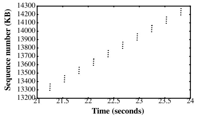
Figure 7. Simulation results showing a portion of the ack trace for the forward transfer after the reverse transfer has started up. ACC is used in conjunction with acks-first scheduling. There is an idle time of about 280 ms between bursts of acks because of the 1 KB data packets belonging to the reverse transfer.
