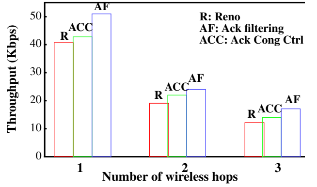
Figure 10. TCP throughputs from simulations of Reno, ACC and AF, as a function of the number of wireless hops.
