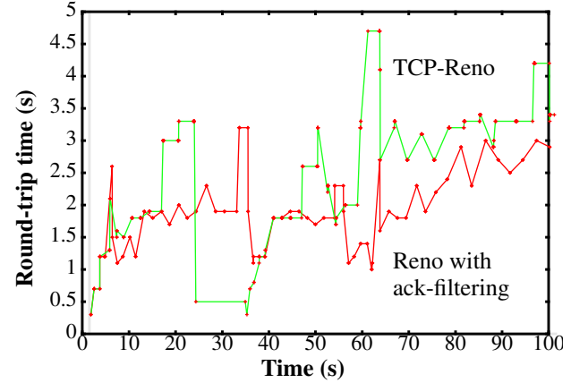
Figure 11. Round-trip times obtained from simulations of TCP Reno and TCP with AF and traffic shaping for a connection over two packet radio hops. The round-trip times for the Reno connection are much more variable, with a mean of 2.67 secs and a standard deviation of 1 sec, whereas AF reduces the mean to 1.85 secs and the standard deviation to 0.6 secs.
