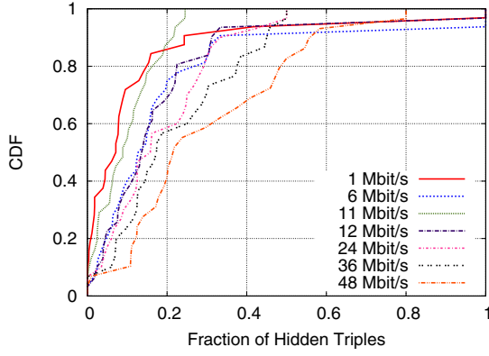
Figure 16: Hidden triples at a threshold of 10%, taking into account the capture effect with a threshold of 10dB.
