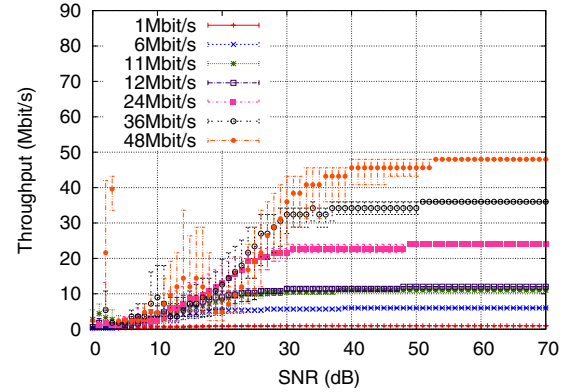
Figure 7: Median throughput versus SNR aggregated across all links in all 802.11b/g networks. Error bars indicate the upper and lower quartiles.
