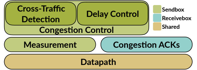
Figure 3: Bundler comprises of six sub-systems: four (in green) implement sendbox functionality, one (in blue) implements receivebox functionality, and the datapath (orange) is shared between the two.
