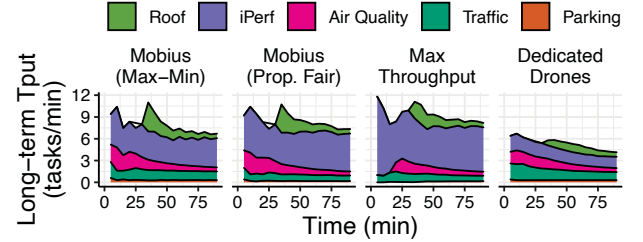
Figure 15: Long-term throughputs achieved over 90 minutes. Mobius achieves high throughput and best shares it amongst the apps.
