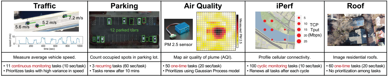
Figure 13: Summary of aerial sensing applications, which span a variety of spatial demand and reactive/continuous sensing preferences. We collected ground truth data for each of these applications using real drones, and created traces to evaluate Mobius.
