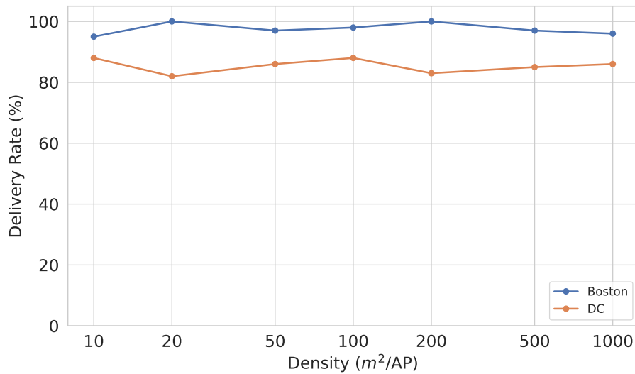
Figure 12 Delivery performance given variation in the simulated density of CityMesh devices in two representative cities. This experiment varies the placement of devices in the city from a device being placed every 10 m^2 to a device every 1000 m^2 . Small fluctuations in the results are attributable to the stochastic placement of devices within building footprints..
