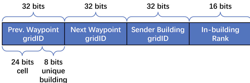
■ Figure 6 CityMesh packet header format.
