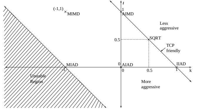
Figure 1. The (k, l) space of nonlinear controls from our family, with the k + l = 1 line showing the set of TCP-compatible controls.
