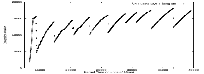
Figure 18. Window variation for a vat session using SQRT congestion control with a bottleneck configured using Dummynet ( b = 50 Kbps, RTT = 900 ms).
