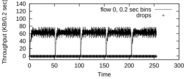
Figure 12. A SQRD flow responding to periods of low loss-rate interspersed with periods of high loss-rate.
