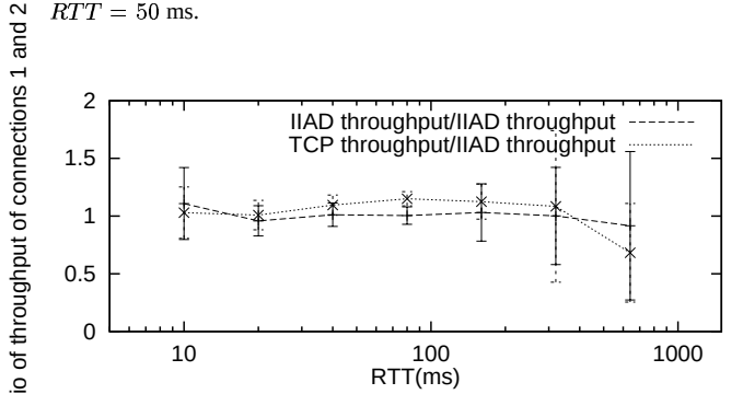
Figure 6. Ratio of throughputs of two connections sharing the bottleneck along with 95% confidence intervals ( n = 10, b = 10 Mbps).
