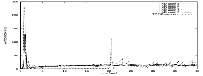
Figure 9. A TCP AIMD connection grabs its fair share of bandwidth in the presence of many long-lived IIAD flows ( n = 16 , b = 9 Mbps, RTT = 50 ms). For clarity, we only show the window sizes of five IIAD connections and the TCP connection.
