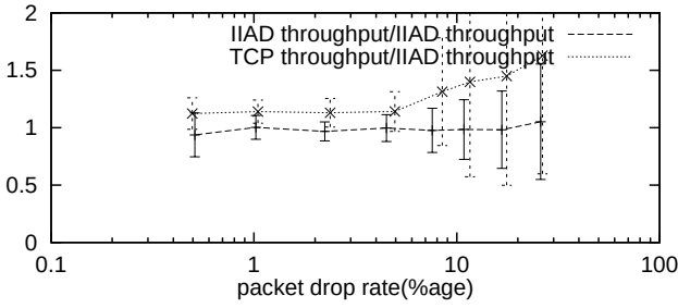
Figure 7. Ratio of throughputs of two connections sharing the bottleneck along with 95% confidence intervals ( n = 10 , rtt = 100ms ).
