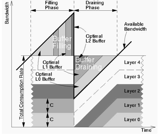
Figure 2. Optimal inter-layer buffer distribution as derived in [17, 19]. Figure from [17], reprinted with permission.
