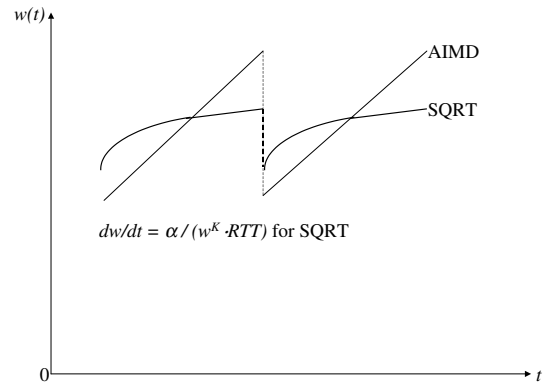
Figure 1. Window evolution vs time for SQRT and AIMD congestion controls. w(t) is the window value at time t .
