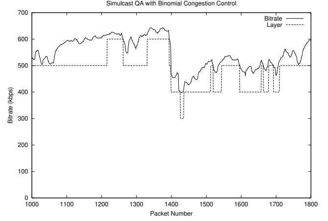
Figure 10. SQRT congestion control with simulcast quality adaptation.
