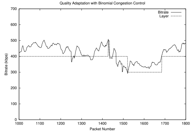
Figure 13. SQRT congestion control for hierarchical encoding with receiver-buffered quality adaptation.
