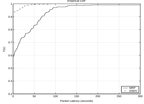
Figure 7: CDF of packet latency for DSDV and MRP-enhanced DSDV for the Random Movement model for a pause time of 60 seconds and 50 nodes.
