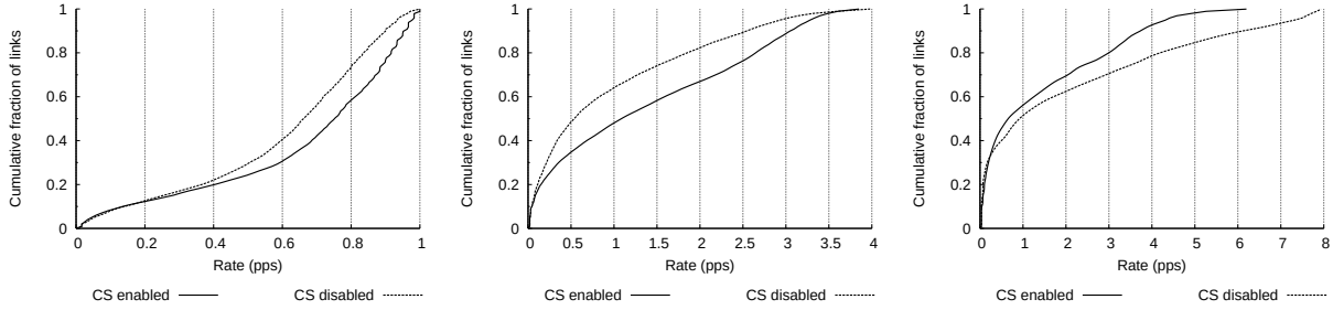
Figure 3: The achieved link throughput distribution in the sensor network when each node offers one pps (left). Duplicate experiments at an offered load of four pps (center) and eight pps (right). Under extreme load, disabling carrier sense improves throughput.
